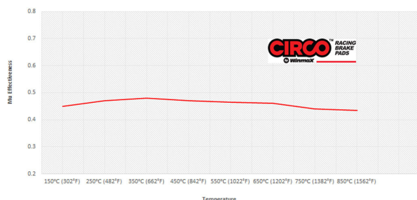
Circo M119 Friction vs Temperature
