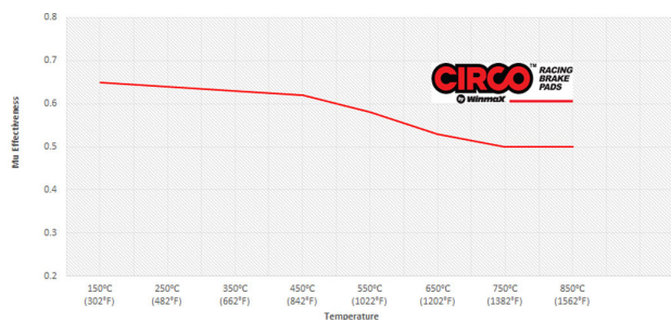
Circo M127 Friction vs Temperature
