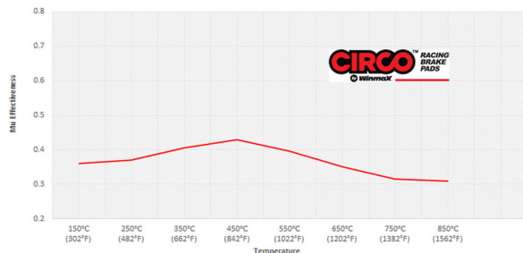
Circo M111 Friction vs Temperature
